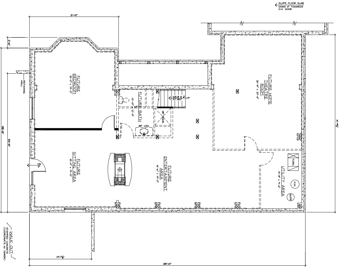
LOWER LEVEL/BASEMENT/FOUNDATION PLAN SCALE 1/4"=1'-0"
