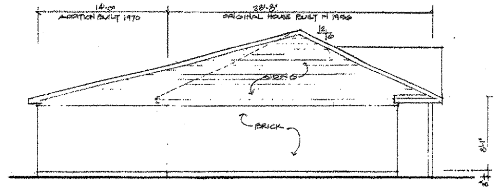
LEFT SIDE ELEVATION 1/4" = 1'-0"
