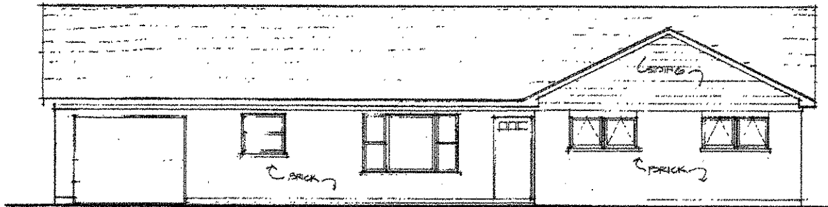
FRONT ELEVATION 1/4" = 1'-0"
